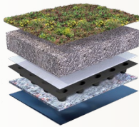
Traditioneel sedumdak
